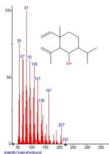
Fig. 20 : Chromatogram of 6-epi-schybunol in Faucheri .
