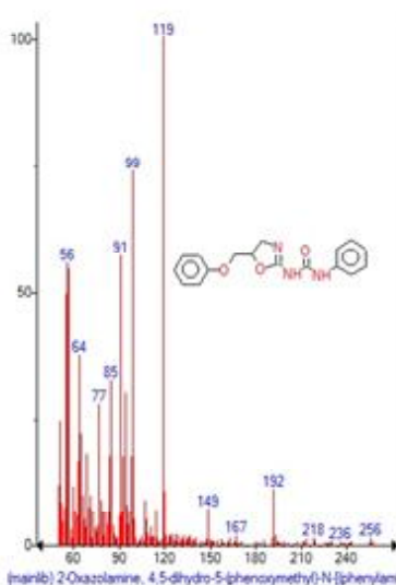
Fig. 12 : Chromatogram of 2-Oxazolamine, 4,5-dihydro-5-(phenoxymethyl)-N-[(phenylamino) in F.aucheri .
