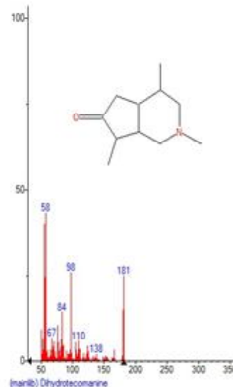
Fig. 13 : Chromatogram of Dihydratecomanine in F.aucheri .
